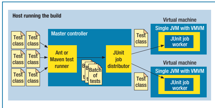
FIGURE 2. The high-level architecture of VMVM (Virtual Machine in a Virtual Machine on a Virtual Machine). Our system integrates directly with test execution initiated by Ant or Maven, or via JUnit directly. Each test class execution is intercepted and sent to a master controller that delegates test cases to workers.
